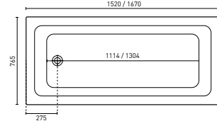
CORTEZ (P. 16) 1520 x 765 x 450 mm (136L) 1670 x 765 x 450 mm (154L)
