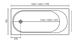
TURIN (P. 15) 1520 x 755 x 445 mm (121L) 1665 x 755 x 445 mm (138L) 1790 x 755 x 485 mm (153L)
