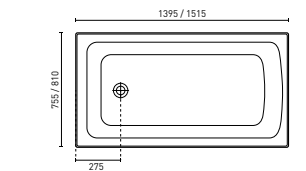
SHENSEKI (P. 16) 1395 x 755 x 480 mm (137L) 1515 x 810 x 520 mm (191L)
