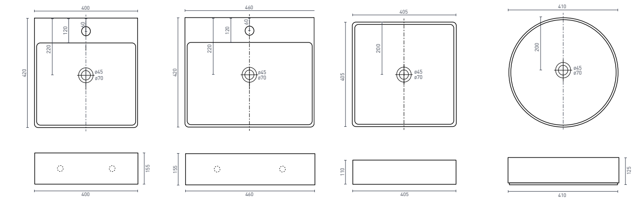
ARIA - Square (p. 10) 400 x 420 x 155 (4.5L)
