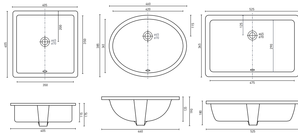
CARINA - Square (p. 10) 405 x 405 x 175 (6.4L)
