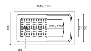
SCARLET (P. 16) 1510 x 815 x 430 mm (124L) 1638 x 815 x 430 mm (159L)
