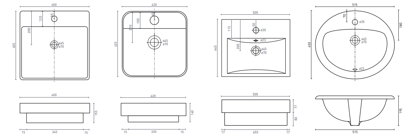
ARIA - Square (p. 12) 400 x 400 x 155 (4.5L)
