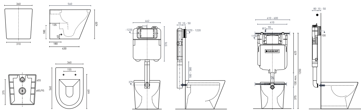
RENEE RIMLESS WALL FACED PAN (p. 6) 560 x 360 x 420 mm - Universal setout 60-90mm
