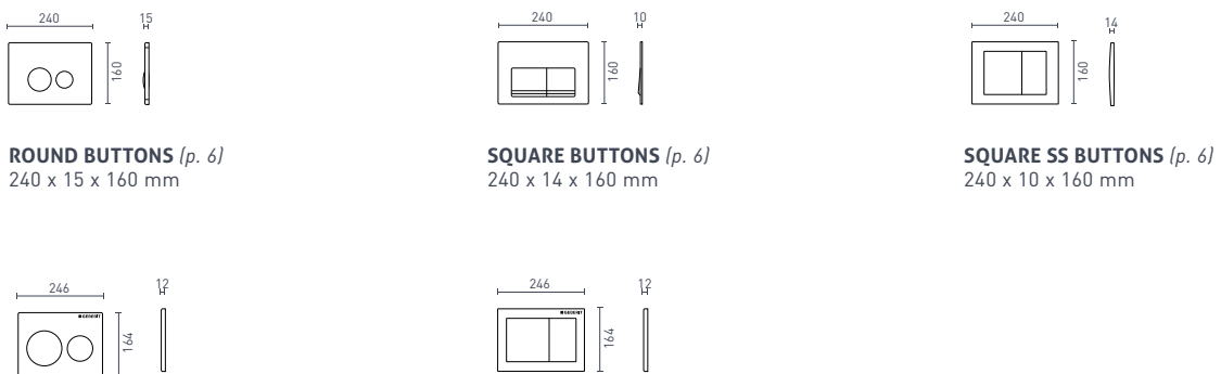
GEBERIT ROUND BUTTONS (p. 6) 246 x 12 x 164 mm
