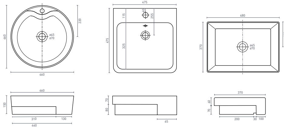
CAVAL - Round (p. 10) 460 x 460 x 150 (5L)
