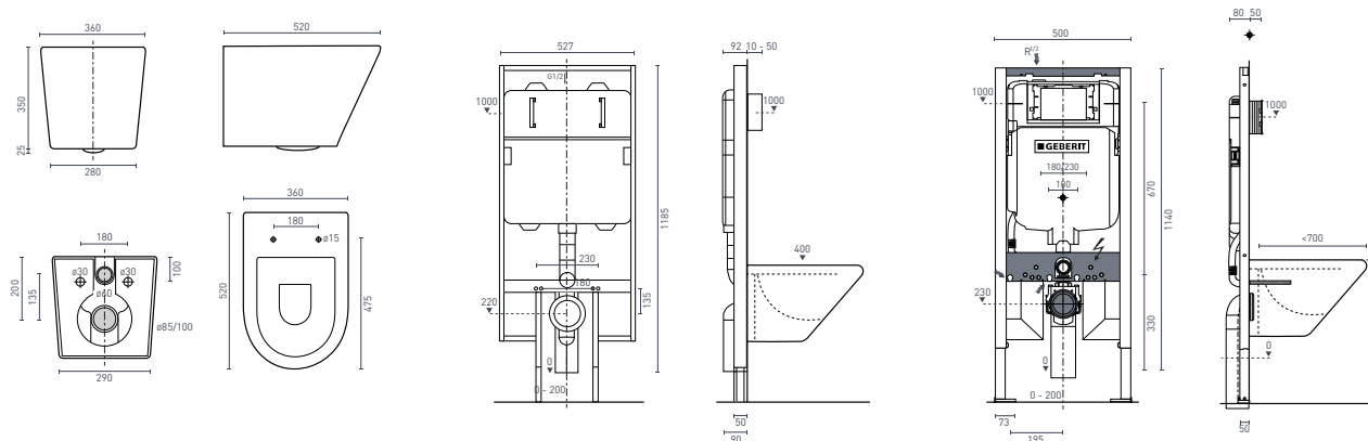
RENEE RIMLESS WALL HUNG PAN (p. 6) 520 x 360 x 375 mm - P-Trap setout 180mm
