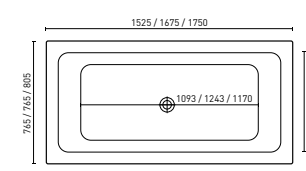
CARINA (P. 17) 1525 x 765 x 440 mm (147L) 1675 x 765 x 440 mm (166L) 1750 x 805 x 480 mm (182L)
