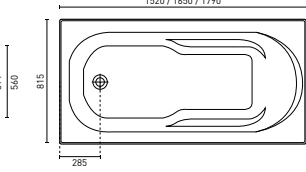
PRIMA (P. 15) 1515 x 815 x 445 mm (124L) 1635 x 815 x 510 mm (159L) 1785 x 815 x 510 mm (194L)
