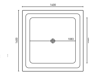
VENICE (P. 17) 1400 x 1400 x 500 mm (370L)
