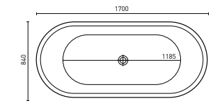
ELISI (P. 12) 1700 x 840 x 595 mm (190L)
