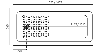
FABRINO (P. 16) 1525 x 765 x 400 mm (130L) 1675 x 765 x 400 mm (154L)
